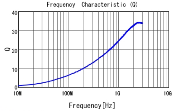
■ LQP15MN5N6B02 Q
