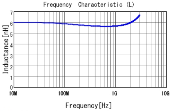
■ LQP15MN5N6B02 L
