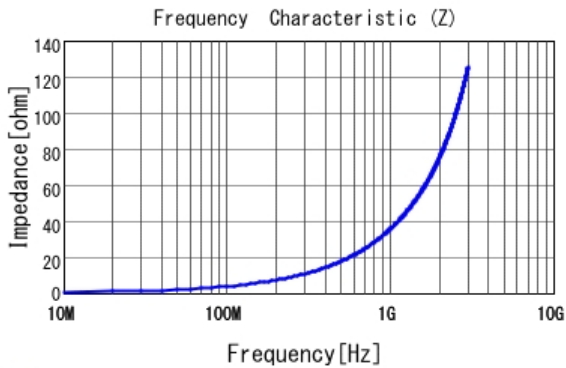
■ LQP15MN5N6B02 |Z|
