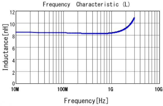
■ LQP15MN8N2B02 L
