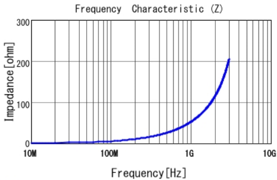
■ LQP15MN8N2B02 |Z|
