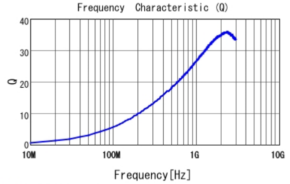
■ LQP15MN8N2B02 Q
