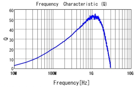
■ LQW15AN82NJ00 Q
