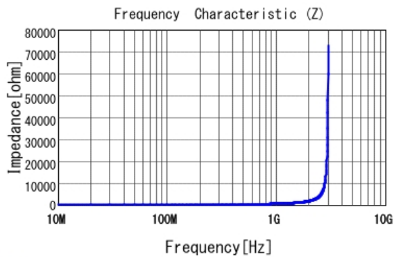
■ LQW15AN82NJ00 |Z|
