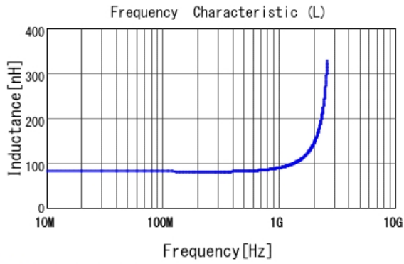
■ LQW15AN82NJ00 L
