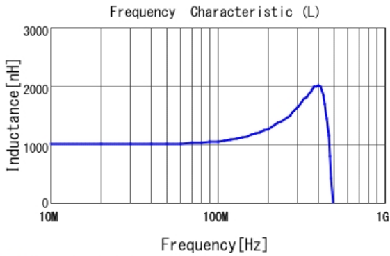
■ LQW21HN1R0J00 L
