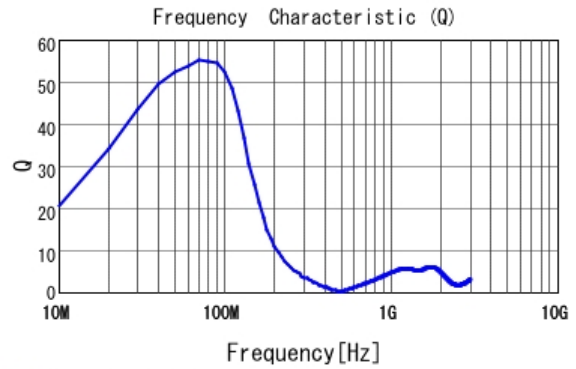
■ LQW21HN1R0J00 Q
