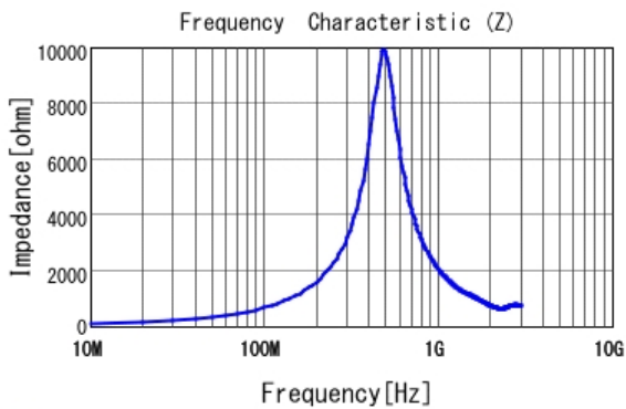
■ LQW21HN1R0J00 |Z|
