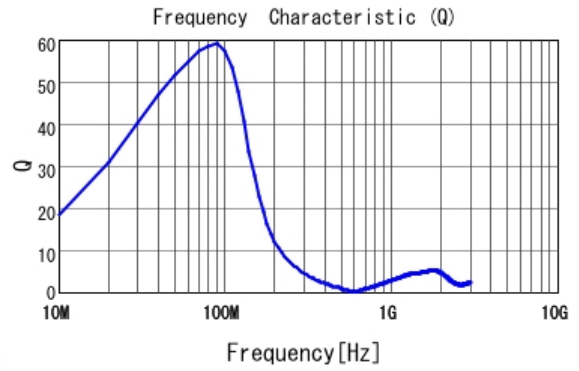
■ LQW21HNR82J00 Q
