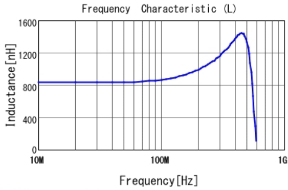
■ LQW21HNR82J00 L
