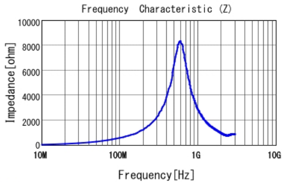
■ LQW21HNR82J00 |Z|
