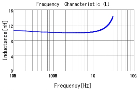
■ LQW2BAS10NG00 L
