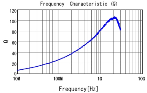
■ LQW2BAS12NJ00 Q
