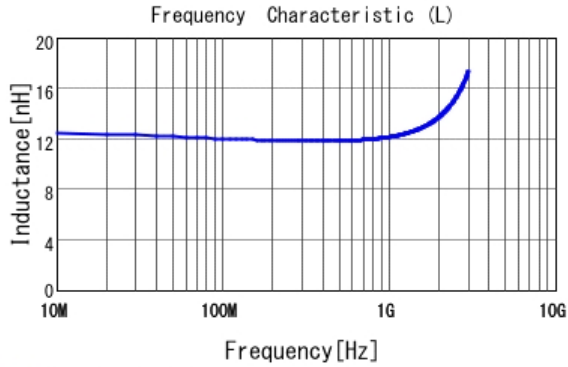
■ LQW2BAS12NJ00 L
