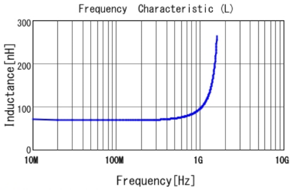
■ LQW2BAS68NJ00 L
