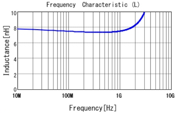
■ LQW2BAS7N5J00 L
