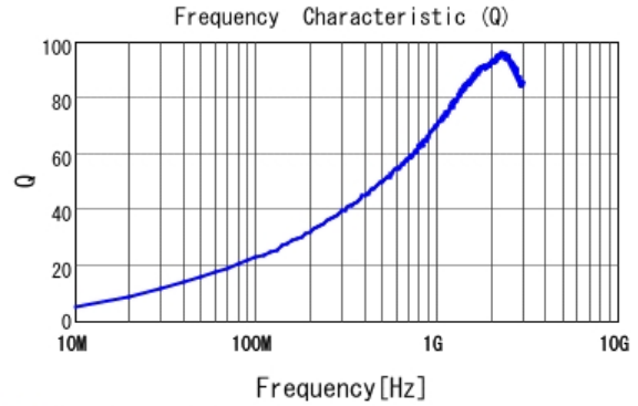
■ LQW2BAS7N5J00 Q
