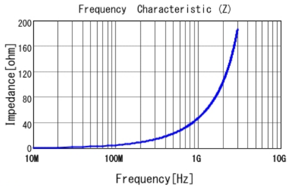
■ LQW2BAS7N5J00 |Z|
