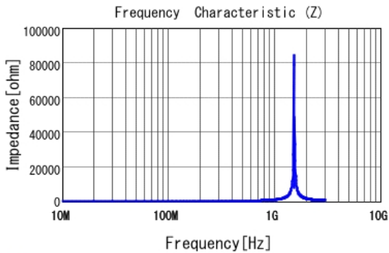
■ LQW2BASR10J00 |Z|
