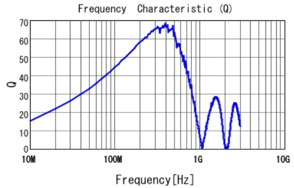
■ LQW2BASR18J00 Q
