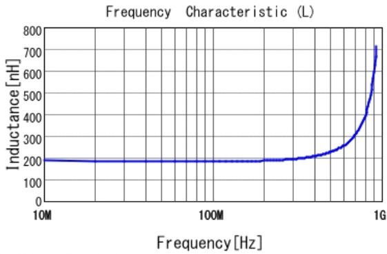
■ LQW2BASR18J00 L
