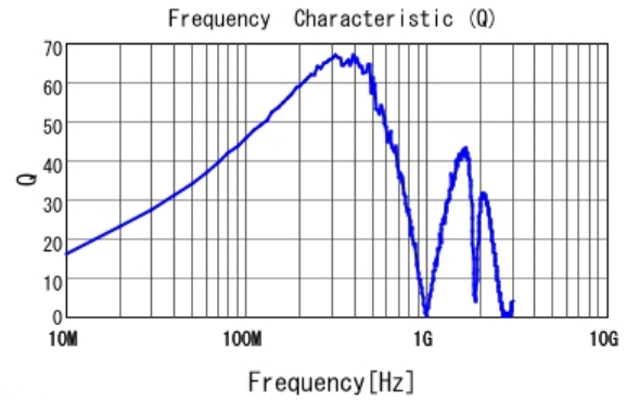
■ LQW2BASR22G00 Q
