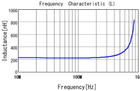
■ LQW2BASR22J00 L
