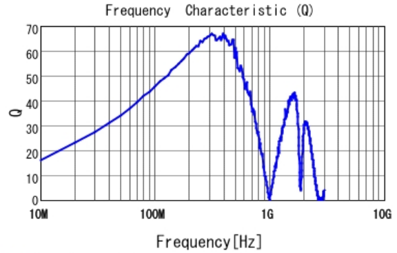
■ LQW2BASR22J00 Q
