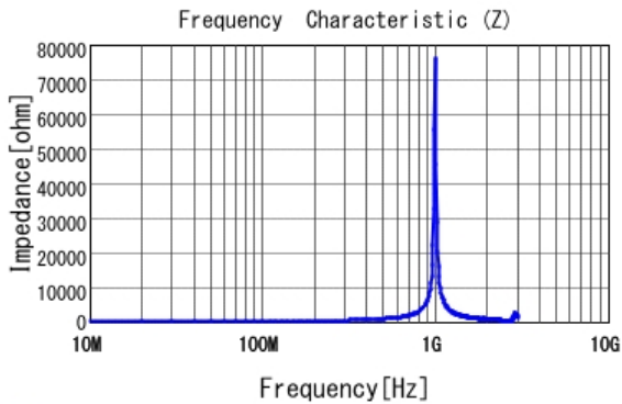
■ LQW2BASR22J00 |Z|
