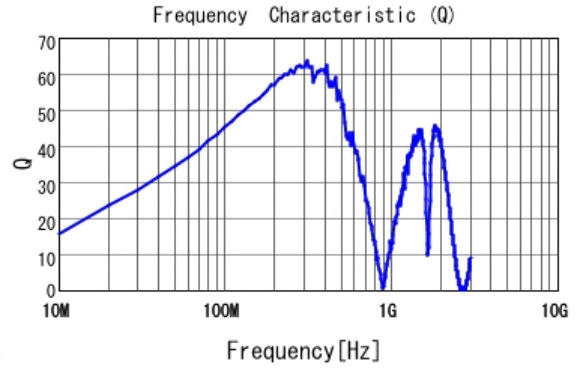
■ LQW2BASR27J00 Q
