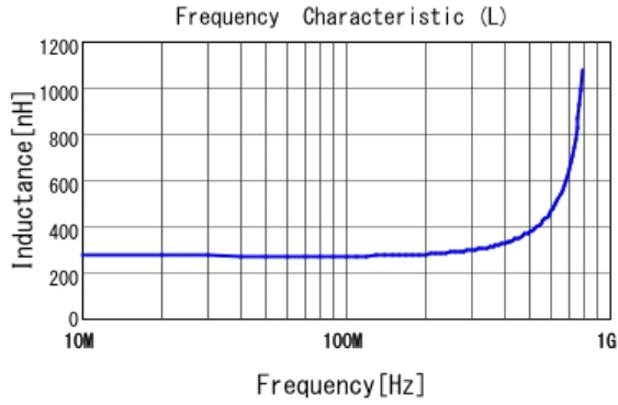
■ LQW2BASR27J00 L
