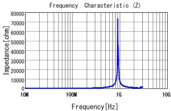
■ LQW2BASR27J00 |Z|
