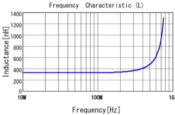
■ LQW2BASR33J00 L
