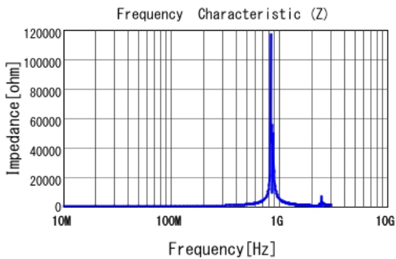
■ LQW2BASR33J00 |Z|
