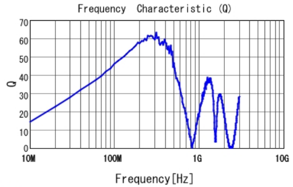
■ LQW2BASR33J00 Q
