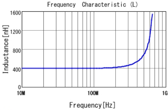
■ LQW2BASR39J00 L
