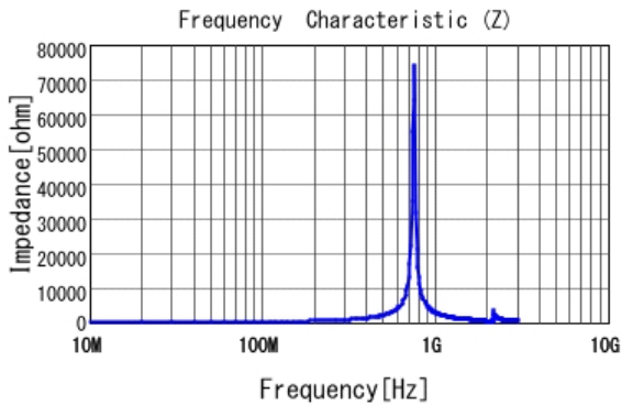
■ LQW2BASR39J00 |Z|
