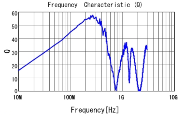
■ LQW2BASR39J00 Q
