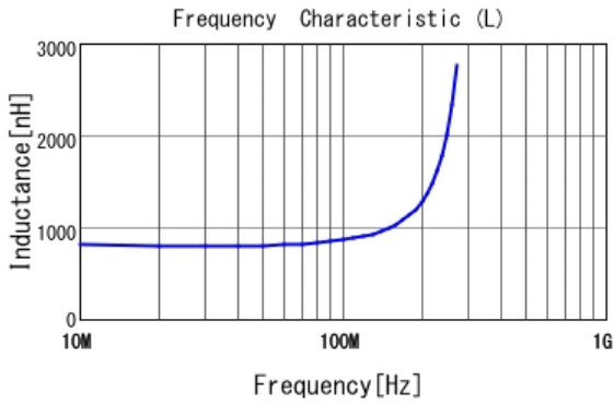
■ LQW2BASR82J00 L
