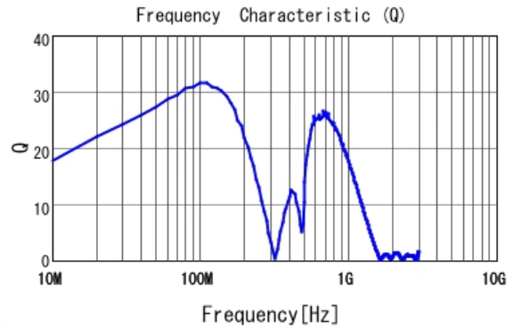
■ LQW2BASR82J00 Q
