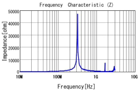
■ LQW2BASR82J00 |Z|
