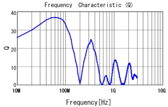
■ LQW2UAS1R8J00 Q
