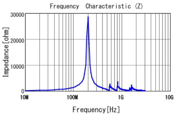
■ LQW2UAS1R8J00 |Z|
