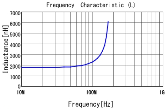
■ LQW2UAS1R8J00 L
