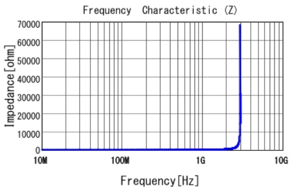
■ LQW2UAS22NJ00 |Z|
