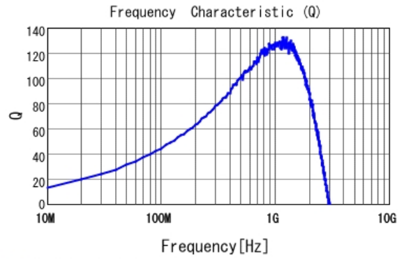
■ LQW2UAS22NJ00 Q
