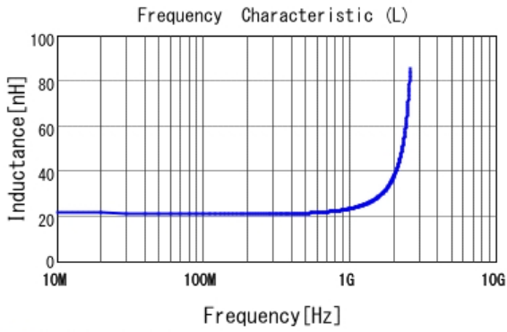
■ LQW2UAS22NJ00 L
