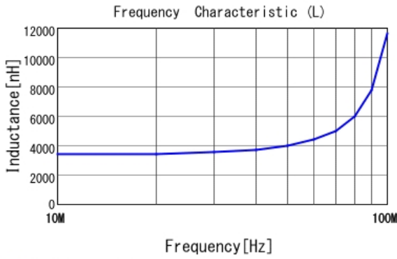
■ LQW2UAS3R3J00 L
