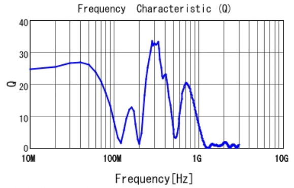
■ LQW2UAS3R3J00 Q
