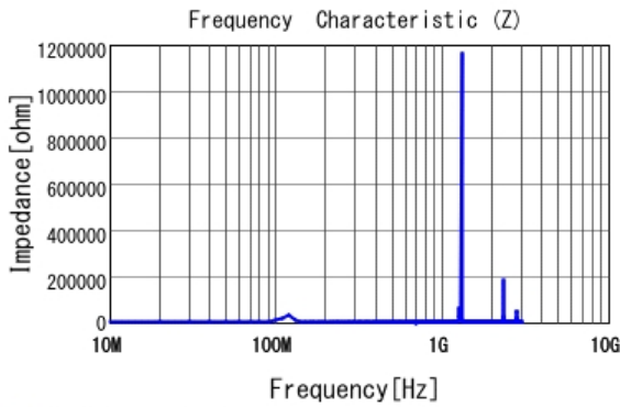
■ LQW2UAS3R3J00 |Z|
