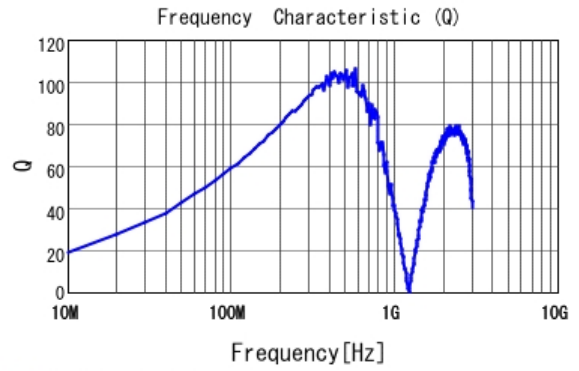
■ LQW2UAS82NJ00 Q
