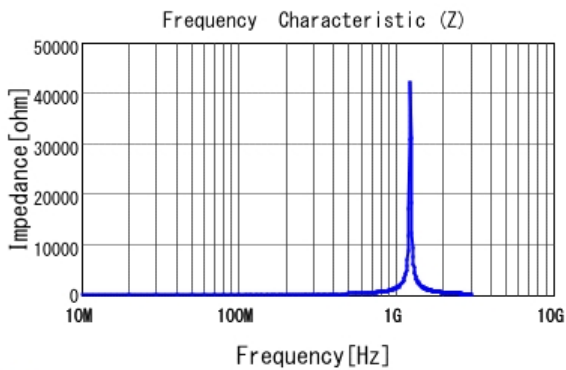
■ LQW2UAS82NJ00 |Z|
