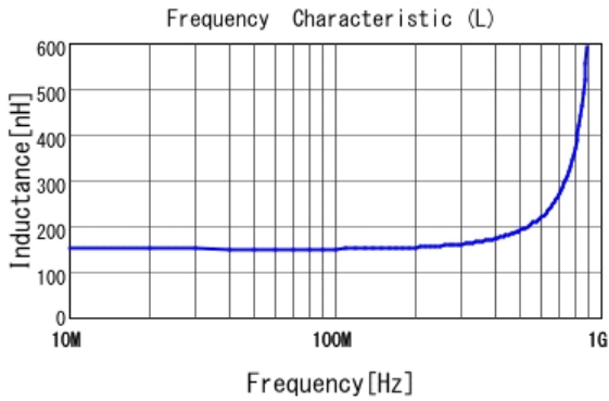
■ LQW2UASR15J00 L
