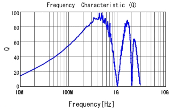
■ LQW2UASR15J00 Q
