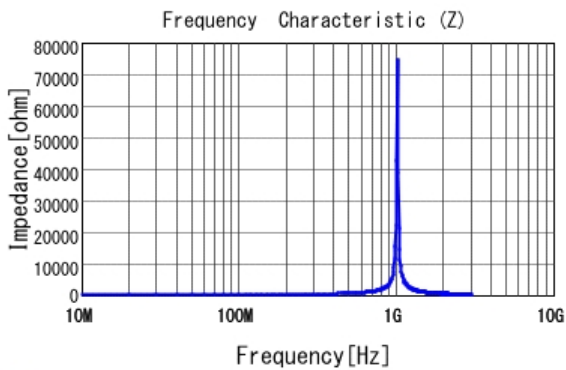
■ LQW2UASR15J00 |Z|
