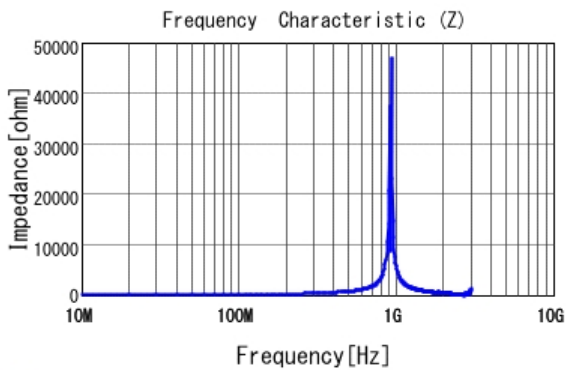
■ LQW2UASR18J00 |Z|
