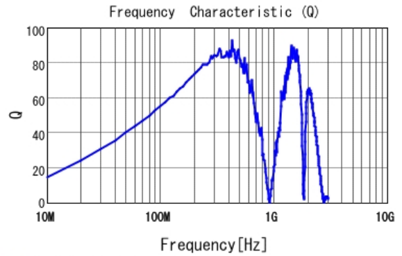
■ LQW2UASR18J00 Q
