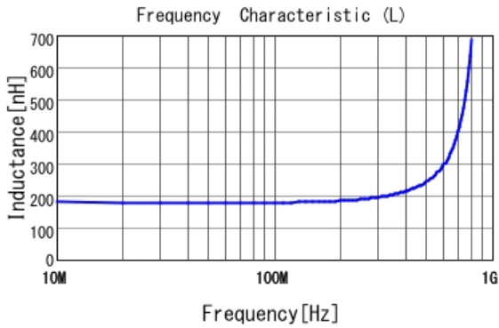
■ LQW2UASR18J00 L
