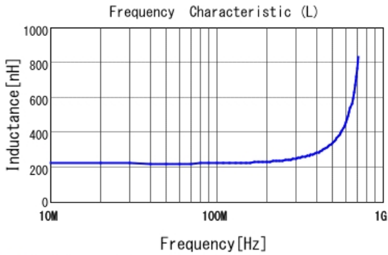
■ LQW2UASR22J00 L
