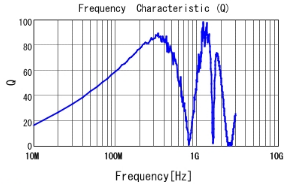
■ LQW2UASR22J00 Q
