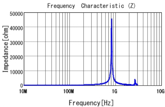
■ LQW2UASR22J00 |Z|
