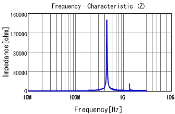
■ LQW2UASR75J00 |Z|
