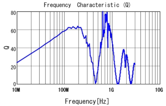
■ LQW2UASR75J00 Q
