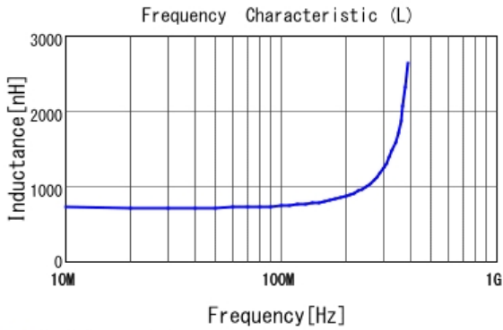
■ LQW2UASR75J00 L
