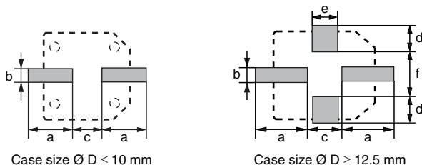
Fig.3 Recommended soldering pad dimensions
