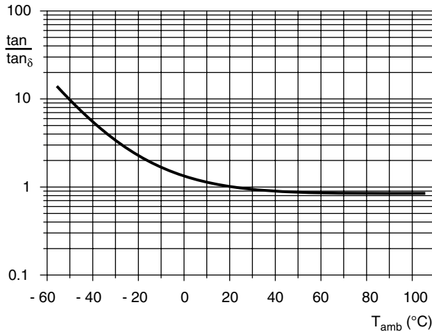
Fig.9 Typical multiplier of dissipation factor tan δ as a function of temperature at 20 °C at 100 Hz tan δ 0 = typical tan δ at 20 °C, 100 Hz
