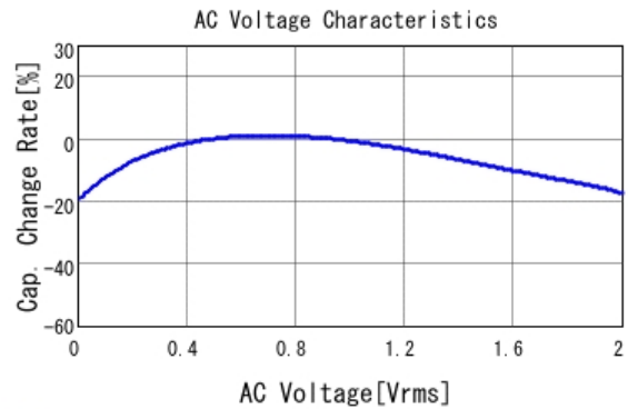
■ NFM15PC435R0G3 C-AC Voltage capchange, DC0V, 25.0degC
