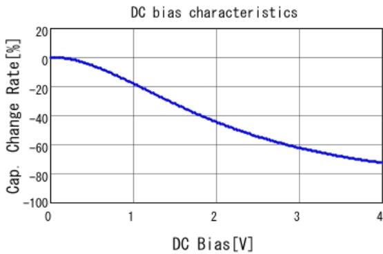
■ NFM15PC435R0G3 C-DC bias capchange, 25.0degC, AC0.5Vr
