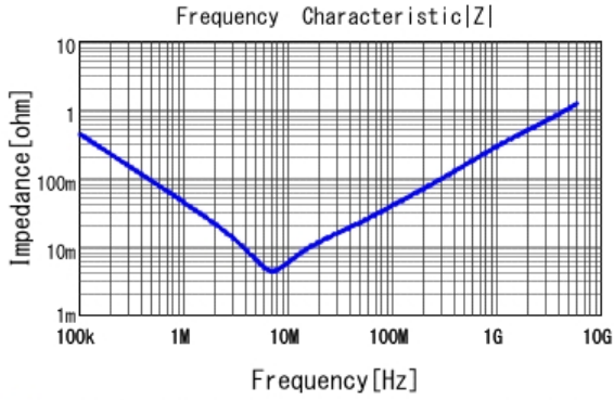
■ NFM15PC435R0G3 |Z| DC0V, 25degC, Non-feedthrough
