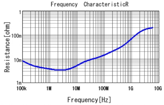
■ NFM15PC435R0G3 R DC0V, 25degC, Non-feedthrough
