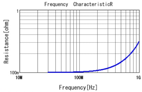
■ RCE5C1H151J0A2H03B R DC0V, 25degC
