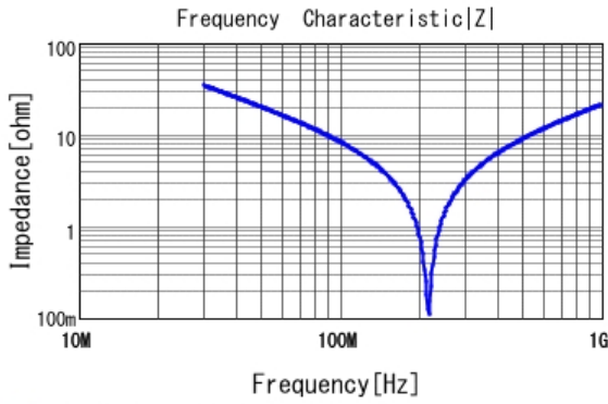
■ RCE5C1H151J0A2H03B |Z| DC0V, 25degC
