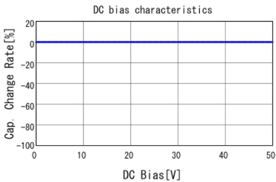
■ RCE5C1H560J0K1H03B C-DC bias capchange, 25.0degC, AC1
