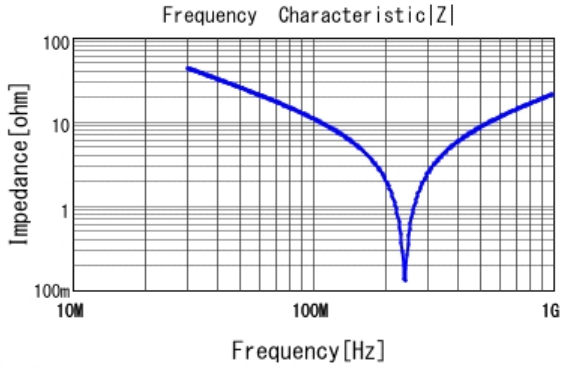
■ RCE5C2A121J0A2H03B |Z| DC0V, 25degC
