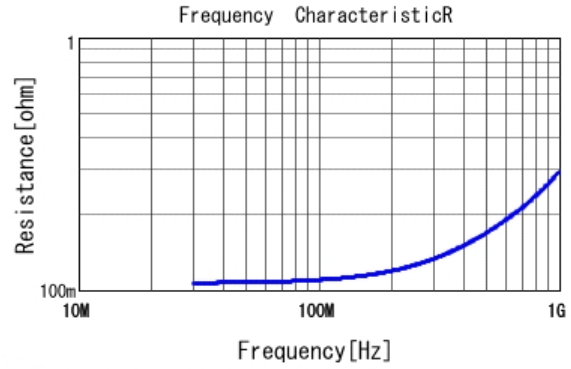
■ RCE5C2A121J0A2H03B R DC0V, 25degC
