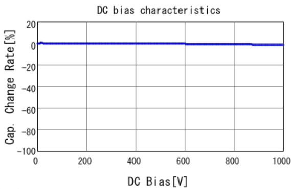
■ RCE7U3A470J2K1H03B C-DC bias capchange, 25.0degC, AC1
