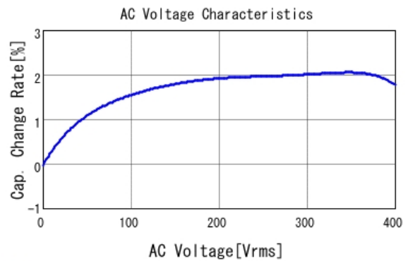
■ RCE7U3A470J2K1H03B C-AC Voltage capchange, DCOV, 25.0
