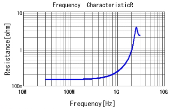
■ RCE7U3A470J2K1H03B R DCOV, 25degC
