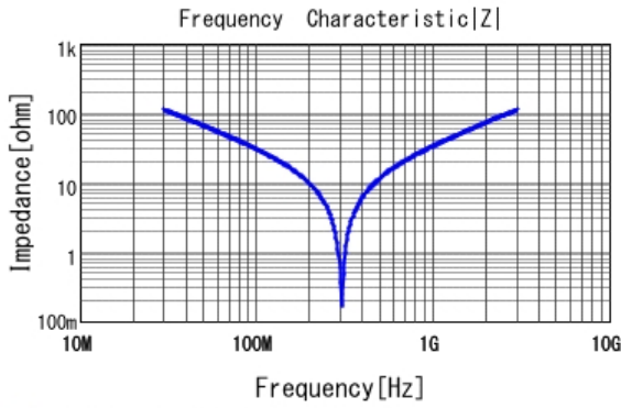
■ RCE7U3A470J2K1H03B |Z| DCOV, 25degC
