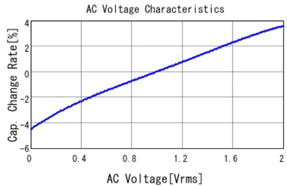
■ RCER71H105K2K1H03B C-AC Voltage capchange, DCOV, 25.0
