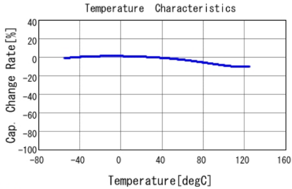
■ RCER71H105K2K1H03B C-Temp. capchange, DC0.0V, AC1.0Vr
