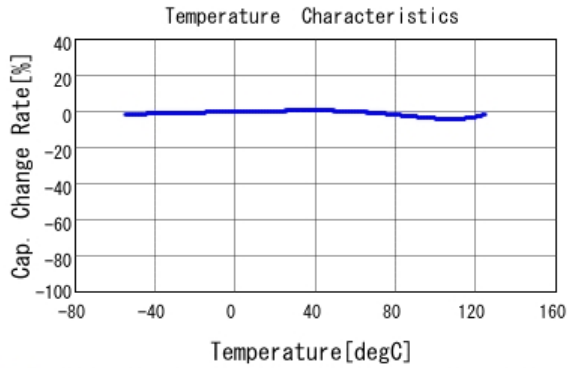
■ RCER71H154K1K1H03B C-Temp. capchange, DC0.0V, AC1.0Vr
