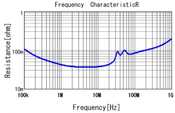
■ RCER71H154K1K1H03B R DC0V, 25degC
