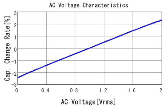
■ RCER71H154K1K1H03B C-AC Voltage capchange, DC0V, 25.0
