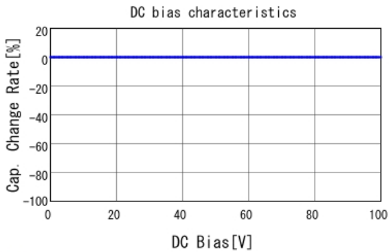
■ RDE5C2A220J0S1H03A C-DC bias capchange, 25.0degC, AC1
