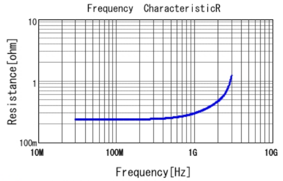
■ RDE5C2A220J0S1H03A R DC0V, 25degC
