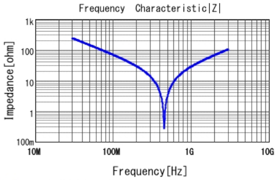
■ RDE5C2A220J0S1H03A |Z| DC0V, 25degC
