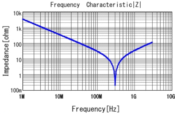
■ RDE7U3A470J2K1H03B |Z| DC0V, 25degC
