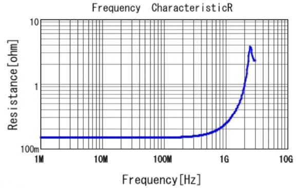
■ RDE7U3A470J2K1H03B R DC0V, 25degC
