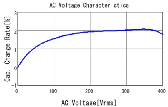
■ RDE7U3A470J2K1H03B C-AC Voltage capchange, DC0V, 25.0
