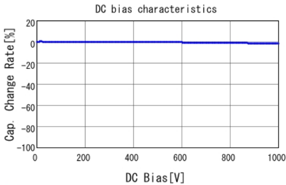
■ RDE7U3A470J2K1H03B C-DC bias capchange, 25.0degC, AC1
