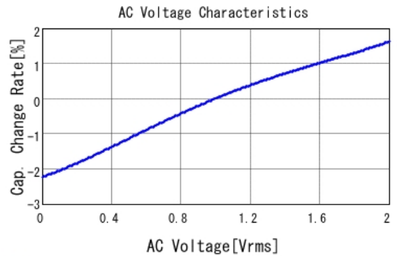
■ RDER71H102K0P1H03B C-AC Voltage capchange, DC0V, 25.0
