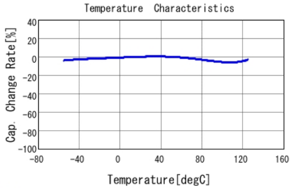
■ RDER71H102K0P1H03B C-Temp. capchange, DC0.0V, AC1.0Vr
