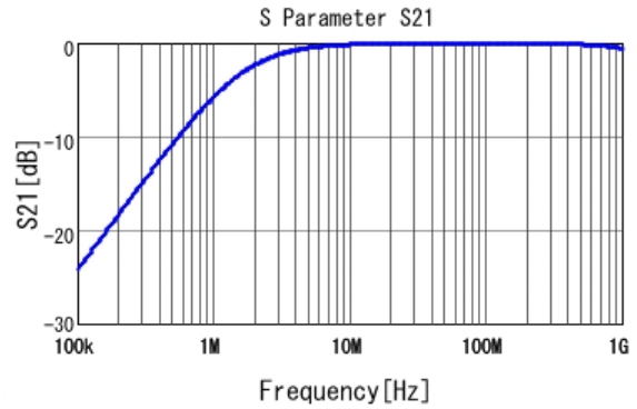
■ RDER71H102K0P1H03B S21 DC0V, 25degC
