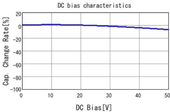
■ RDER71H102K0P1H03B C-DC bias capchange, 25.0degC, AC1
