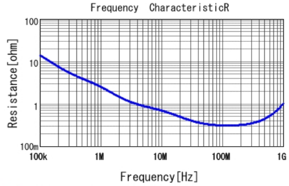
■ RDER71H102K0P1H03B R DC0V, 25degC
