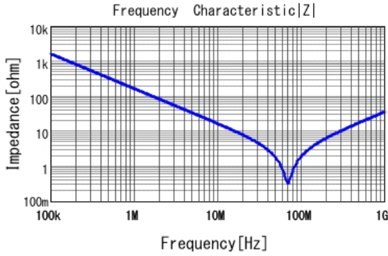
■ RDER71H102K0P1H03B |Z| DC0V, 25degC
