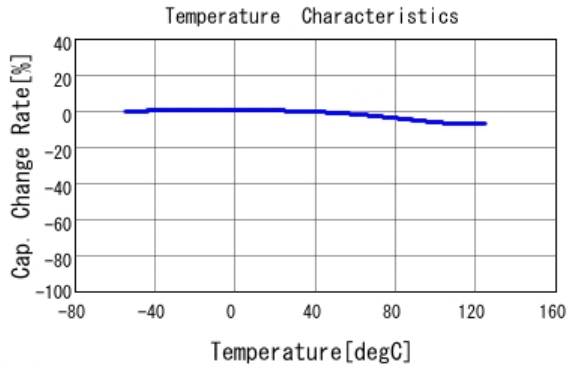
■ RDER71H104K0K1H03B C-Temp. capchange, DC0.0V, AC1.0Vr
