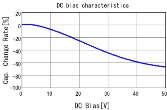
■ RDER71H225K2K1H03B C-DC bias capchange, 25.0degC, AC1
