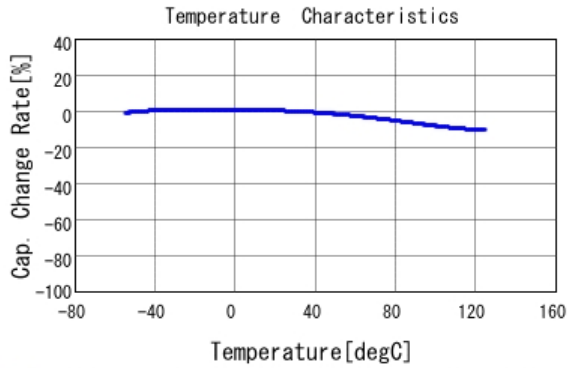
■ RDER71H225K2K1H03B C-Temp. capchange, DC0.0V, AC1.0Vr
