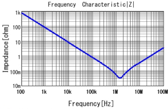
■ RDER71H225K2K1H03B |Z| DCOV, 25degC
