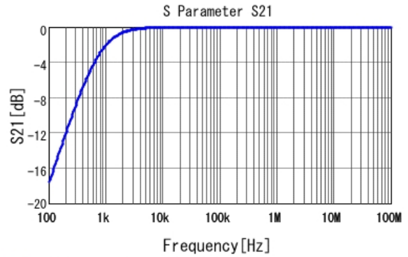
■ RDER71H225K2K1H03B S21 DC0V, 25degC
