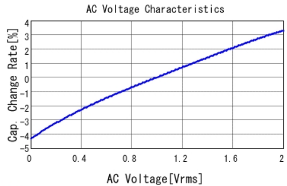
■ RDER71H225K2K1H03B C-AC Voltage capchange, DCOV, 25.0
