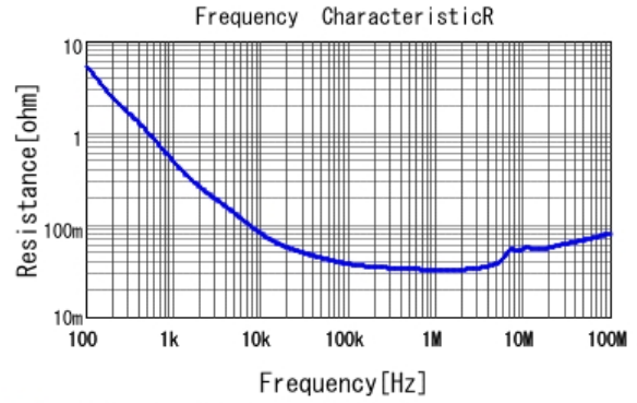
■ RDER71H225K2K1H03B R DCOV, 25degC
