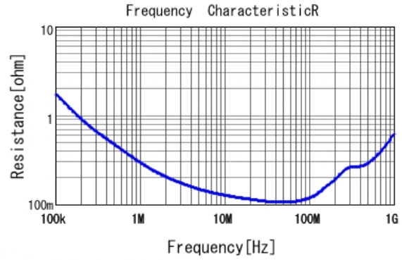
■ RDER72E103K1K1H03B R DCOV, 25degC
