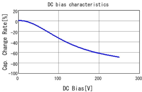
■ RDER72E103K1K1H03B C-DC bias capchange, 25.0degC, AC1
