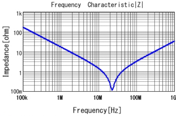
■ RDER72E103K1K1H03B |Z| DCOV, 25degC
