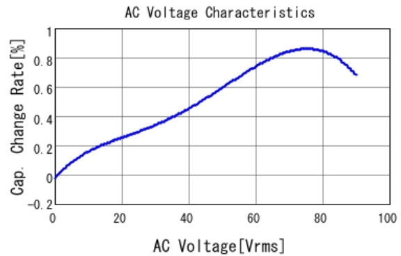
■ RDER72E103K1K1H03B C-AC Voltage capchange, DCOV, 25.0
