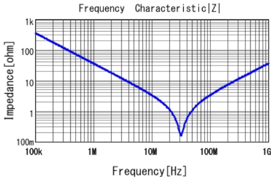
■ RDER73A472K2K1H03B |Z| DC0V, 25degC
