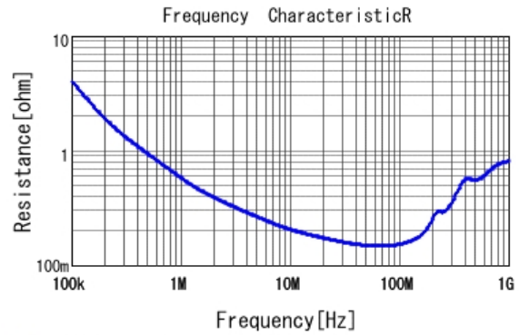
■ RDER73A472K2K1H03B R DC0V, 25degC
