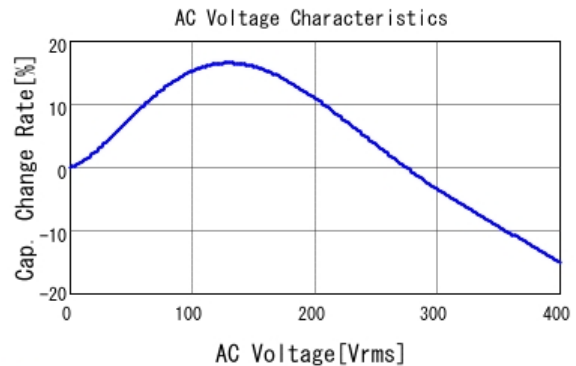
■ RDER73A472K2K1H03B C-AC Voltage capchange, DC0V, 25.0
