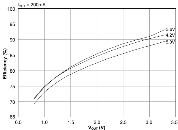
Efficiency vs. V_{OUT} ( T_A = 85^\circ C )
