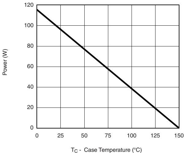
Power, Junction-to-Case
