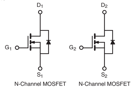
N-Channel MOSFET
