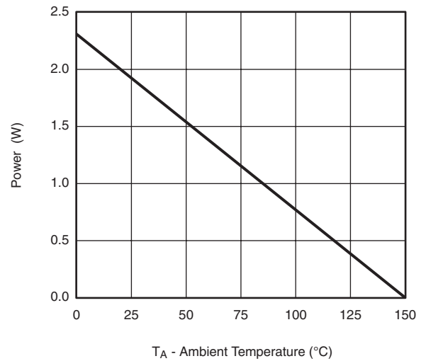
Power, Junction-to-Ambient
