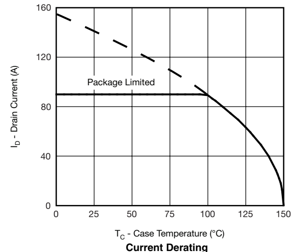
Current Derating
