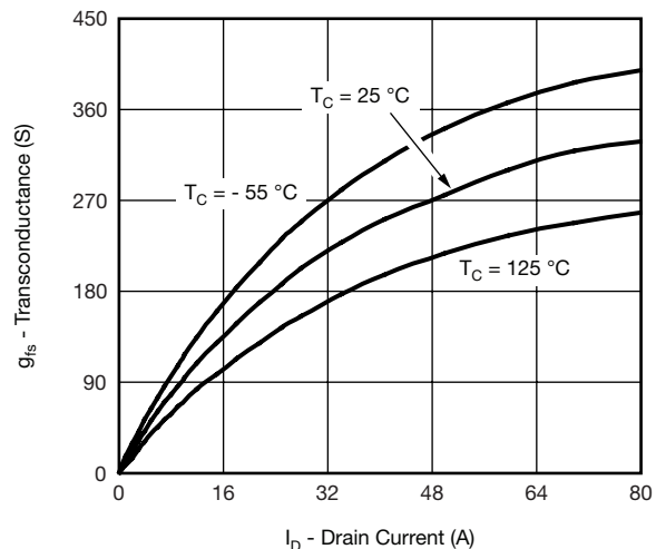
Transconductance
