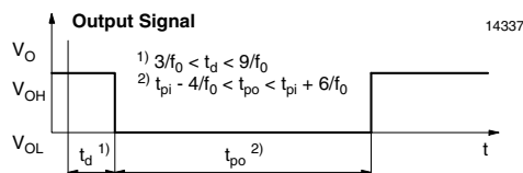
Fig. 1 - Output Active Low
