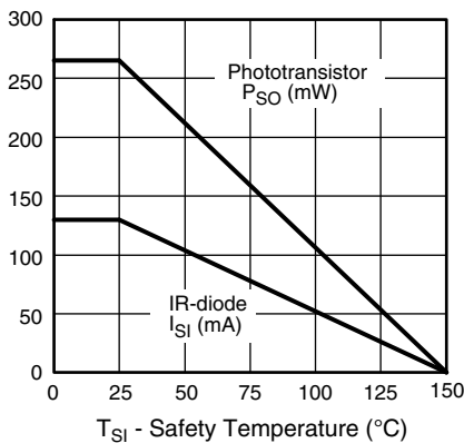
Fig. 1 - Derating Diagram
