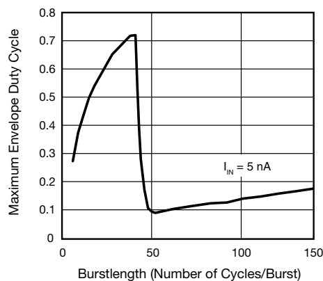
Fig. 7 - Maximum Envelope Duty Cycle
