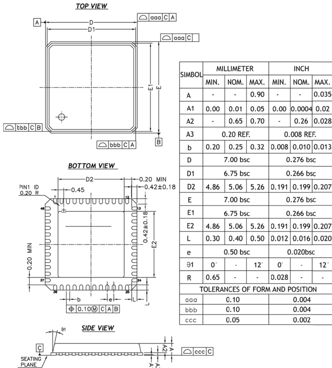
Figure 26 Package Dimensions
