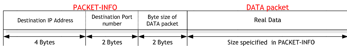
Figure 12 The Received UDP data Format
