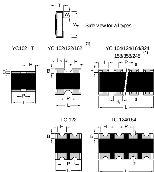
Fig. 12 YC/TC122 series chip resistors dimension Note: I. YC102/104 is flat type
